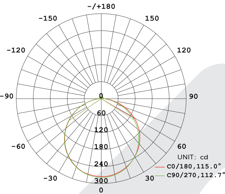
Light distribution
