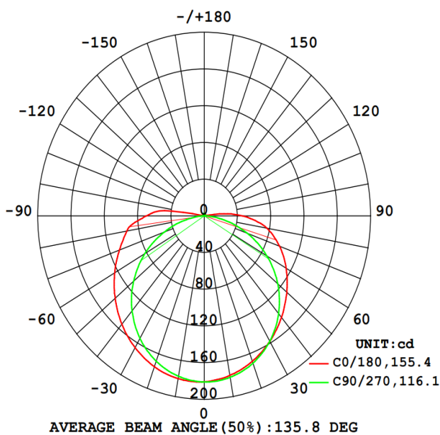
Photometric of 1M (4000K) strip
